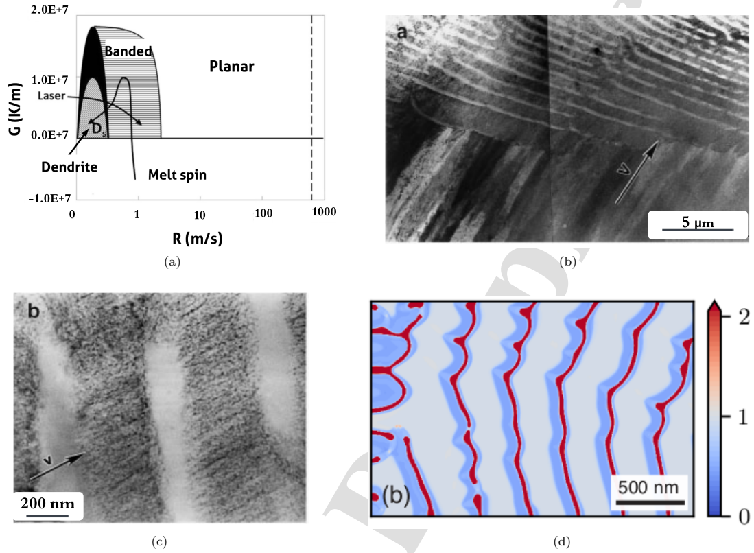
Figure 12: (a) G - R solidification microstructure selection (SMS) map for typical values of G = 10^6 K/m and R = 0.4 m/s, adapted from [180]. (b, c) TEM images of banded structure formation in laser AM of metal alloys (reproduced from [177], with permission from Elsevier). (b) Transition from lamellar eutectic morphology to banded structure (upper part) and vice versa is observed in a eutectic Al-33 % Cu alloy for R = 0.5 m/s. (c) Formation of cellular/dendritic (dark band) and plane front (clear band) banded structure in Al-4 % Fe alloy with R = 0.7 m/s. (d) Phase-field simulation of banded microstructure in Al-9 %Cu alloy is shown using a composition colormap (reproduced from [179], with permission from APS). The band spacing in simulation ( \approx 400 nm) agrees well with the experiment. Composition is represented in mass fraction.
