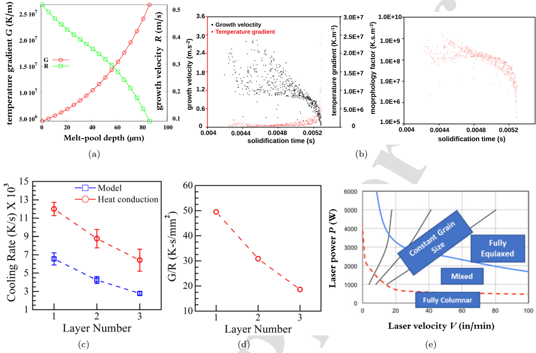
Figure 7: (Color online) (a) FEA simulations estimate G and R in Ti-6Al-4V for P = 200 W and V = 500 m/s, which vary as a function of melt-pool location [93, 94]. (b) FEA simulations compute different solidification parameters that vary as a function of solidification time. Each point in this plot corresponds to a finite element node within a cross-section of the melt-pool (adapted from [63], with permission from Elsevier). (c, d) FEA simulations estimate decreasing cooling rate and morphology factor with increasing layer number in a multi-layer laser AM process (reproduced from [82], with permission from AIP Publishing). (e) Schematically shown how an AM process map describes the solidification microstructure characteristics as a function of P and V (adapted from [29], with permission from Elsevier). This process map combined with the G - R solidification map (Fig. 2a) demonstrate that the length scale and final microstructure can be controlled by exploring these material-specific maps.
