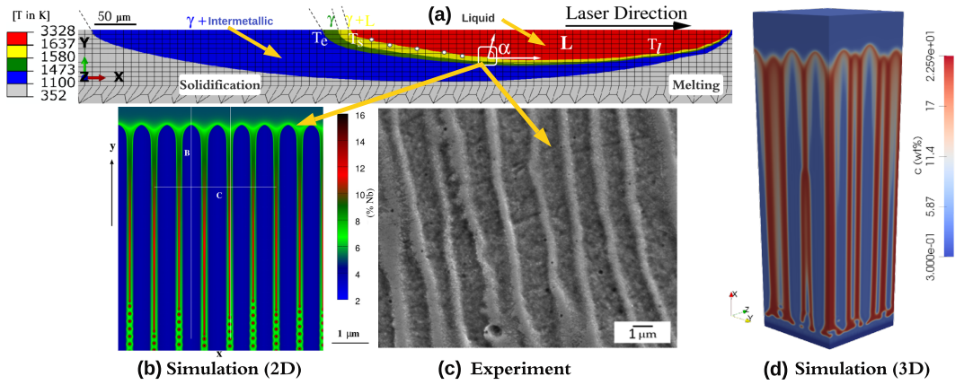
Figure 5: (Color online) Previous work on LPBF of Inconel 625 and 718 alloys [50, 58, 91]. (a) The temperature distribution in the melt-pool was estimated through 3D FEA simulations of a single-track laser scan across a layer of Inconel 718 powder [54]. The laser melt-track is a 2D slice of 3D FEA simulations. The laser power P is 180 W and the beam speed V is 800 mm/s. The values of G and R are determined at different microscopic locations along the mesoscale melt-pool boundary. Here, the temperature boundaries (delineated by different colors) represent various phase transformations, which correspond to the alloy phase diagram. L is liquid, \gamma is the primary solidification phase, and the intermetallic, in general, represents the interdendritic segregated phases that form during terminal solidification. The macroscopic V can be linked to microscopic interface velocity R through V \cdot \cos \alpha , where \alpha is the angle between the velocities. The G at a melt-pool location can be calculated by \|\nabla T\| . (b) The computed G and R values are input to PF simulations, resulting in a cellular microstructure with non-equilibrium composition distribution (shown by the color scale bar); these microscale features are expected to form at the same solidified melt-pool region in AM experiments. (c) Exemplary experimental measurement of cellular microstructure relates to PF simulations (reproduced from [92], with permission from Elsevier). (d) 3D PF simulation of a cellular microstructure with the composition scale bar are shown for the same G and R values as in 2D (Fig. 5b).
