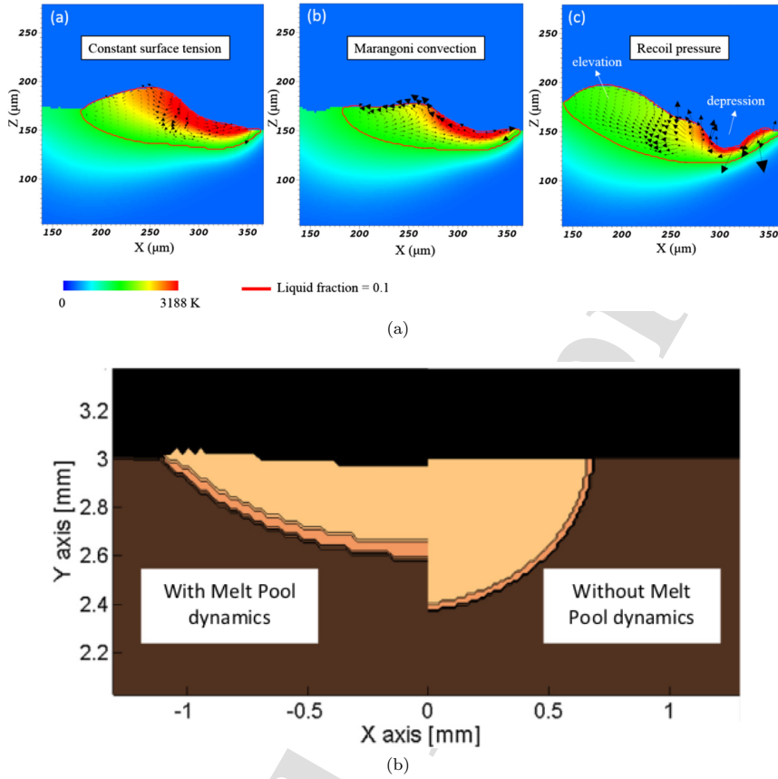
Figure 6: (Color online) (a) In Inconel 625, melt-pool characteristics are simulated under different physical effects but with the same AM parameters and time. These macroscale physical effects modify the mesoscale melt-pool boundary and consequently the estimated solidification parameters (reproduced from [71], with permission from Elsevier). The scale bar denotes temperature. (b) In 304 stainless steel, the influence of the fluid flow on final melt-pool geometry is illustrated (reproduced from [70], with permission from Elsevier). This affects the resulting solidification parameters, which, in turn, determine the evolution of microstructure and defects. All the above laser melt-tracks are 2D slices of 3D FEA simulations.
