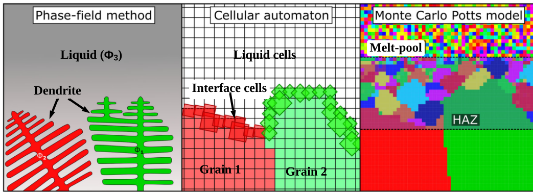
Figure 4: (Color online) Schematic demonstrates the basic idea behind the microstructure simulations using various modeling approaches. With a significantly higher resolution of both the simulation domain and the solid-liquid interface, the phase-field method generates a substantially lower mesh anisotropic error when compared to the cellular automata method. The Potts Kinetic Monte Carlo (KMC) model shows the highest level of abstraction with respect to the physical processes observed during melt-pool solidification with dendrites, segregation, and undercooling are not considered. The KMC method is primarily used to simulate grain evolution during AM [49]. HAZ in the figure (right) stands for the heat affected zone in the material. Adapted from Ref. [14].
