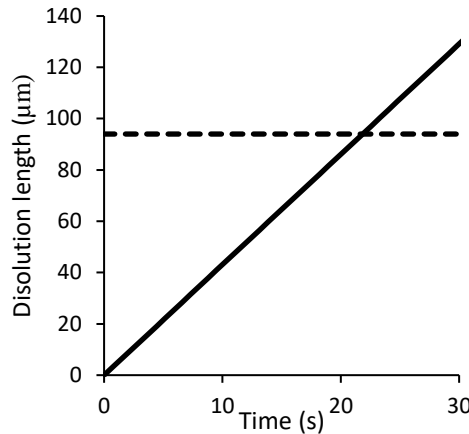
Figure 6: Calculated dissolution over time for TiAlNb rod in TiAl at 1600°C
