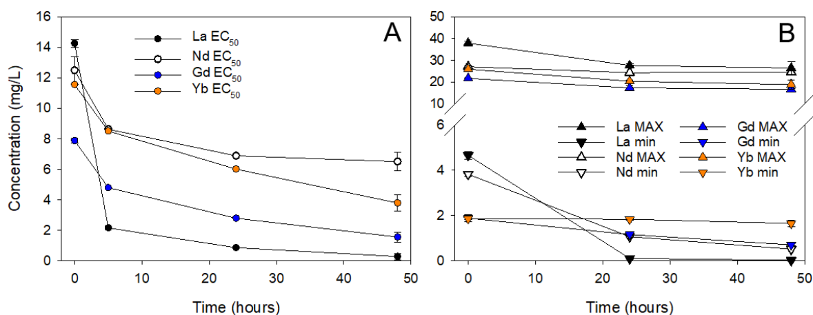
Figure 2. (A) Temporal changes in the filterable concentrations ( < 0.45 \mu\text{m} ) of La, Gd, Nd, Yb for solutions initially amended with lanthanides concentrations equal to the corresponding EC 50 at 24 h. The selected elements are representative of the three different behaviors across the whole lanthanides series (see text for details and Table S9 and Fig. S2 for full results). Measurements at t=0 and t=48\text{h} were performed in duplicate. (B) Same as panel A, but for solutions initially amended with maximum (MAX) and minimum (min) tested concentrations. All measurements performed in duplicate. Error bars may be smaller than the corresponding symbols.
