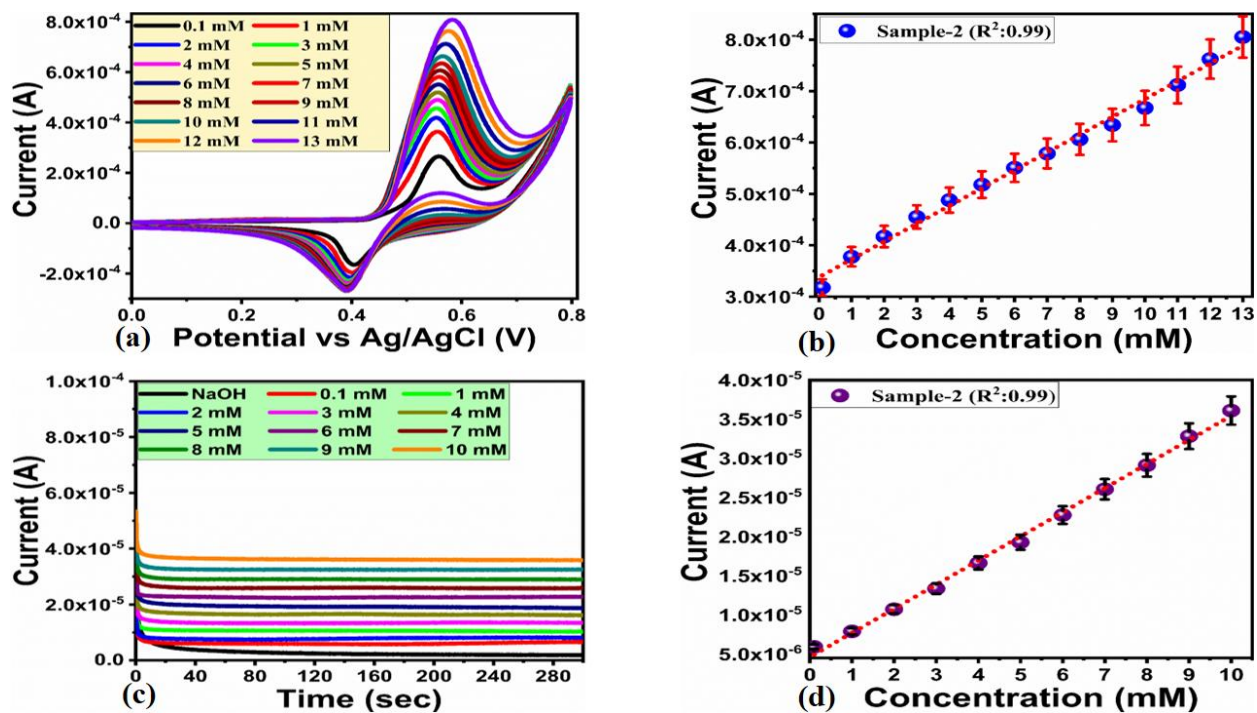
Figure 6. (a) CV curves of sample 2 at 50 mV/s in various urea concentrations prepared in 0.1M NaOH, (b) Linear plot of oxidation peak current against different urea concentrations, (c) Chronoamperometric response of sample 2 against different concentrations of urea, (d) Linear plot of oxidation peak current versus different urea concentrations.
