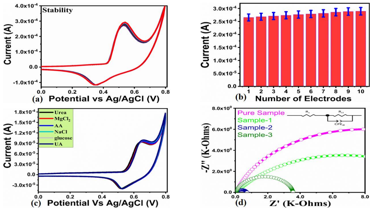
Figure 7. (a) CV curves at 50 mV/s illustrating the repeatable stability of sample 2 in 0.1mM urea, (b) Reproducibility of various modified electrodes of sample 2 in 0.1mM urea, (c) CV curves at 5 mV/s of sample 2 in the different interfering environment of measuring the selectivity, (d) EIS Nyquist plots of different NiO samples in the frequency range of 100000 kHz to 0.1Hz using 0.6V, an amplitude of 5 mV in 0.1mM urea.
