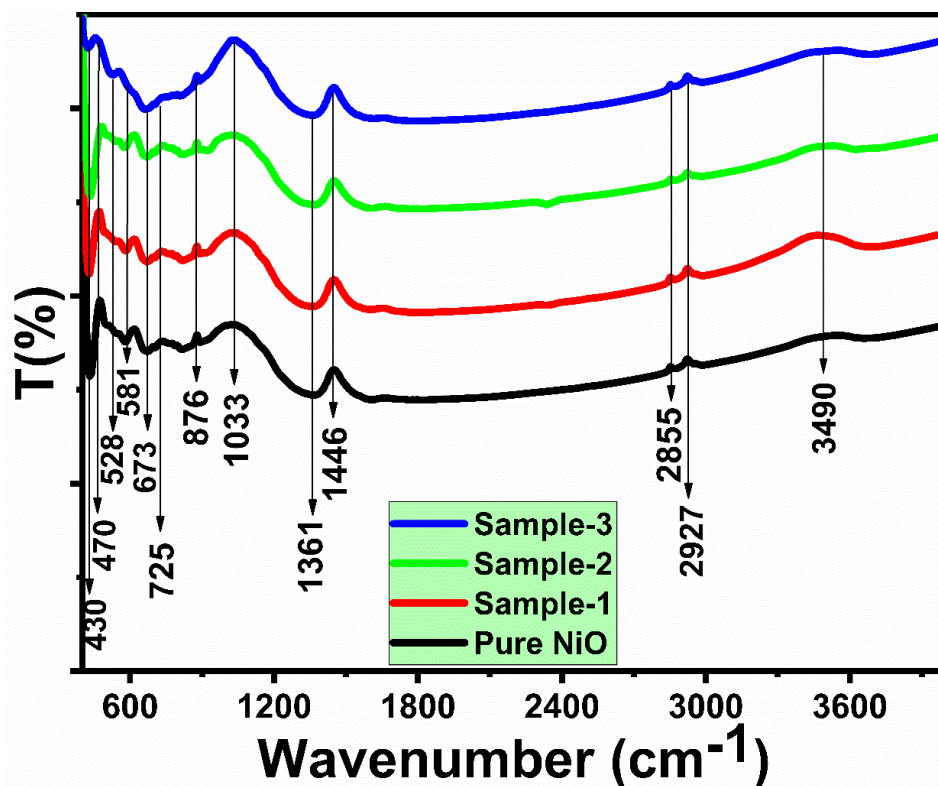
Figure 4. FTIR spectra of various NiO nanostructures prepared with different amounts of wheat pee extract (sample 1, sample 2, and sample 3) and their comparison with pure NiO.
