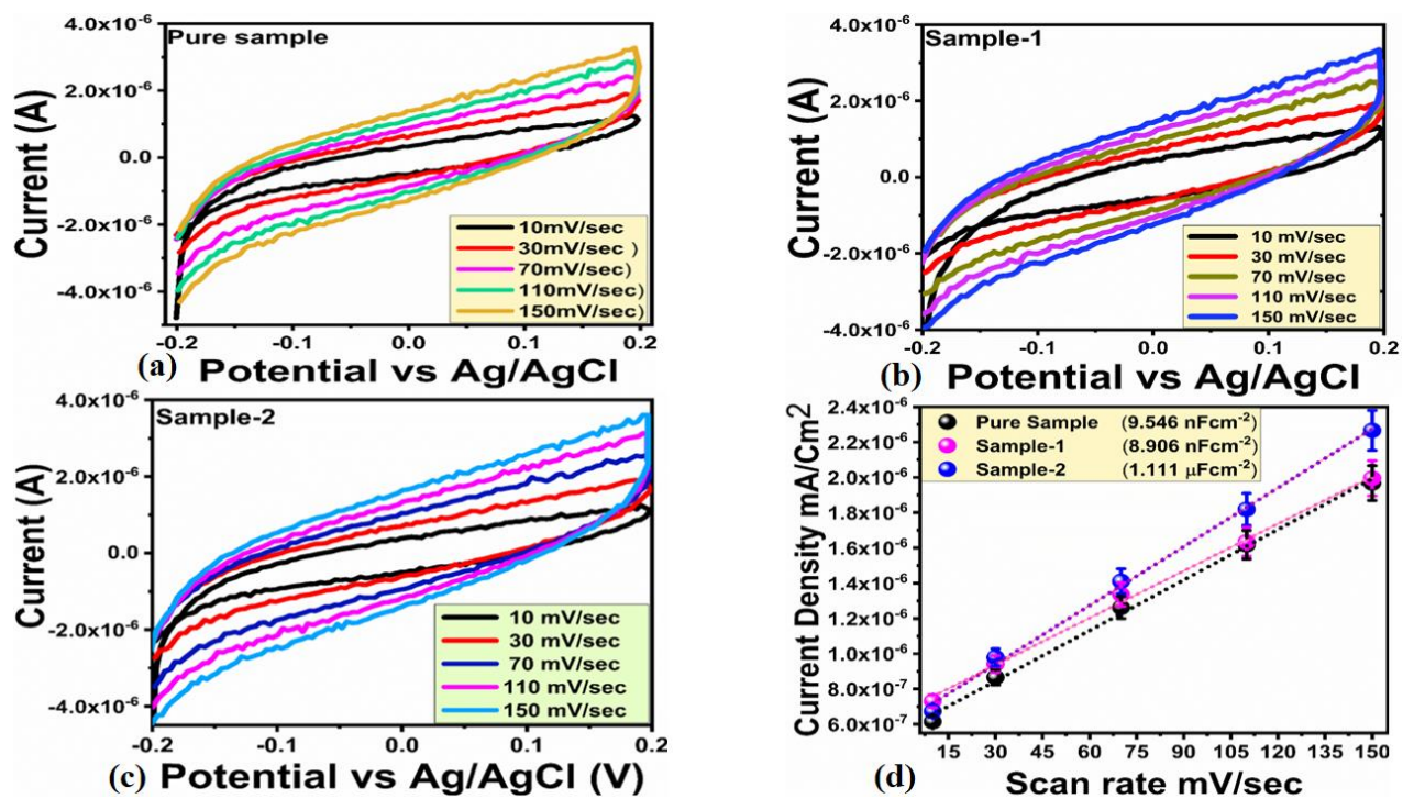
Figure 8. (a-c) Non faradic cv curves of various NiO nanostructures at different scan rates in, 0.1mM urea, (d) Linear plot of the difference of anodic and cathodic sides current densities against scan rate for the quantification of ECSA.
