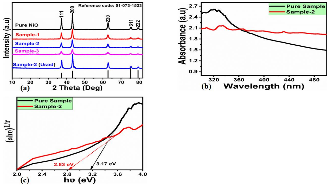
Figure 1. (a) XRD diffraction patterns of pure NiO nanostructures and different amounts of wheat peel extract assisted NiO nanostructures (sample 1, sample 2, and sample 3) and used sample 2, (b) UV-Visible absorbance spectra of pure NiO and the optimized sample 2, (c) Corresponding optical band Tauc plot.
