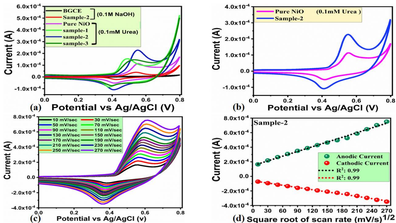
Figure 5. (a) CV curves of bare glassy carbon electrode (BGCE), pure NiO nanostructures and green mediated NiO nanostructures using different volume of wheat peel extract such as 3 mL, 5 mL, 7 mL (sample 1, sample 2, and sample 3) at 50 mV/s with and without urea in 0.1M NaOH, (b) CV curves of pure NiO nanostructures and green mediated NiO nanostructures (sample 2) only measured at 50 mV/s in 0.1mM urea, (c) CV curves of green mediated NiO nanostructures (sample 2) measured at various scan rates in 0.1mM urea, (d) Corresponding linear plot of anodic and cathodic peak currents against square root of scan rate.
