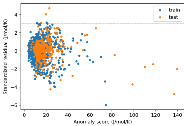
(a) Split 1
