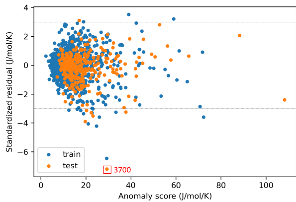
(b) Split 2
