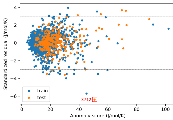
(e) Split 5
