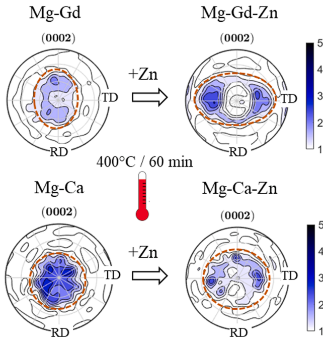
Fig. 1. Comparison of the texture development in Mg-Gd-(Zn) and Mg-Ca-(Zn) alloys upon annealing at 400 °C for 60 min. The color coding for the texture intensities is displayed in terms of multiples of a random distribution. The outlined areas in the (0002) pole figures denote the texture spread with respect to the RD and TD directions.
