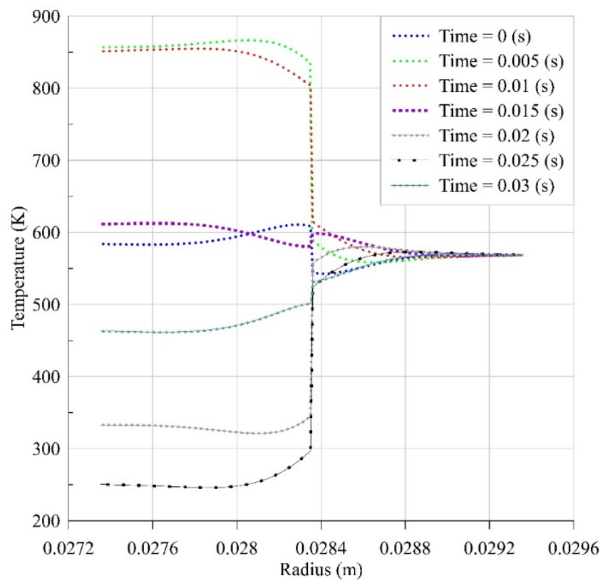
Figure 8. Flow temperature in the gap = 10 μm.
