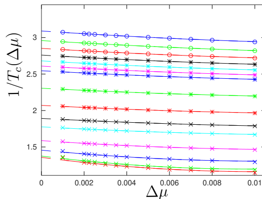
Figure 11. Inverse pseudo-transition temperatures 1/T_c(\Delta\mu) versus \Delta\mu . The different curves correspond to different monomer chemical potentials \mu_1 = -10, -4, -2, -1, -0.4, -0.2, 0, 0.16, 0.26, 0.28, 0.30, 0.32, 0.34, 0.36 and 0.38 (from bottom to top). The continuous curves are quadratic fits of the data.
