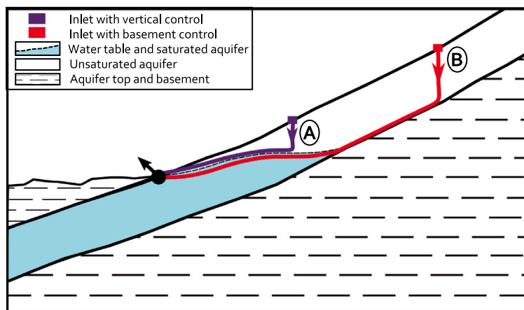
Fig. 5. Cross section in a simple karst aquifer, with two karst conduits with different contexts in the vadose zone: one with vertical control (in purple) and one with basement control (in red). The non-planar water table is also represented with a dashed line. (For interpretation of the references to color in this figure legend, the reader is referred to the web version of this article.)
