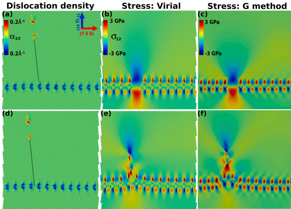
Fig. 7. Interaction between an extrinsic edge dislocation and a \Sigma 291(13\bar{1}\bar{1})[1\bar{1}\bar{2}] low angle STGB in copper, with two scenarios: the edge dislocation will annihilate with one composing the GB (a, b, c); the edge dislocation will stop nearby the GB (d, e, f). Figures (a, d) show the per-atom Nye dislocation density \alpha_{23} in the initial (unrelaxed) configuration for both scenarios. The presence of two positive \alpha_{23} distributions indicates a dissociation of the extrinsic dislocation into Shockley partials. The dashed black lines indicate the \{111\} glide plane of the extrinsic edge dislocation. In (b, e) is shown the per-atom virial stress \sigma_{12} of the final (relaxed) configuration, when the edge dislocation has interacted with the GB, for both scenarios. Figures (c, e) show the same stress fields obtained via application of the G method with a 0.5 \text{ \AA} FFT grid resolution.
