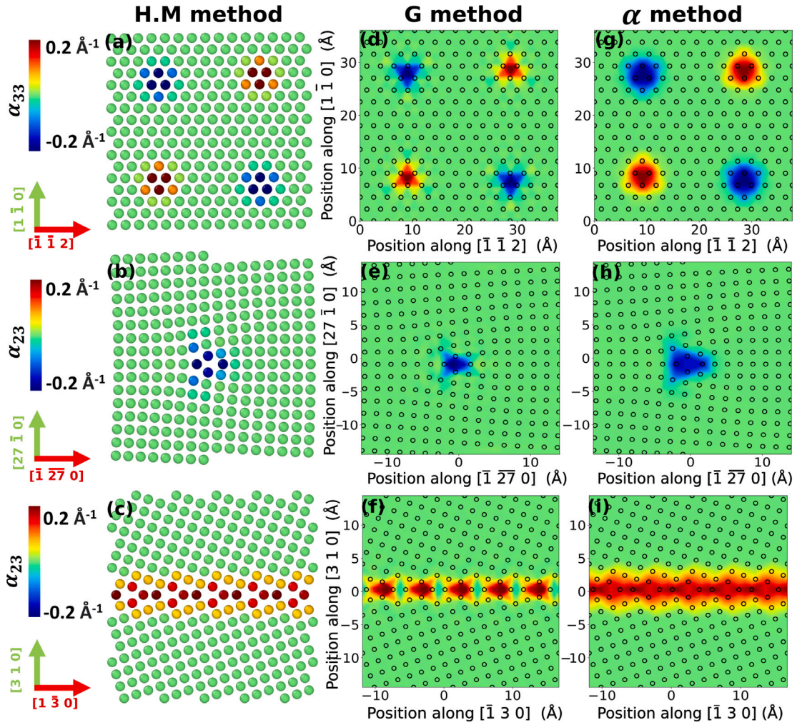
Fig. 3. Comparison of Nye dislocation density distributions obtained with the G and \alpha transfer methods using a 0.5 \text{ \AA} FFT grid resolution. (a), (b) and (c) Visualization of the component \alpha_{33} and \alpha_{23} of the Nye tensor for the screw dislocation quadruple in tungsten, structural units within LAGB and HAGB in copper respectively after atomistic relaxation. (d), (e) and (f) Represent maps displaying the screw and edge dislocation densities obtained via the G method. (g), (h) and (i) show the same densities obtained with the \alpha method.
