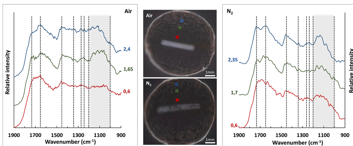
Fig. 6. Visible images of a radial section of tobacco stick heated under air or nitrogen with the areas outlining the FT-IR measurement regions ( 200 \mu\text{m} \times 200 \mu\text{m} ) at different distances from the lamella (mm).
