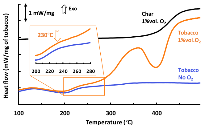
Fig. 11. Comparison between the calorimetry signals for thermal degradation of tobacco under inert (non-oxidative) and oxidative atmospheres and char (produced after tobacco pyrolysis in the calorimeter) under an oxidative atmosphere in a fixed bed configuration.
