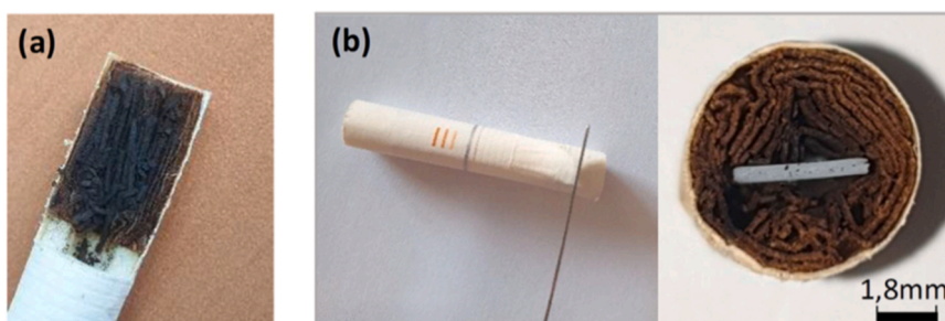
Fig. 2. Longitudinal (a) and radial (b) sections of tobacco sticks with the Teflon mold positioned in lieu of the heating lamella.
