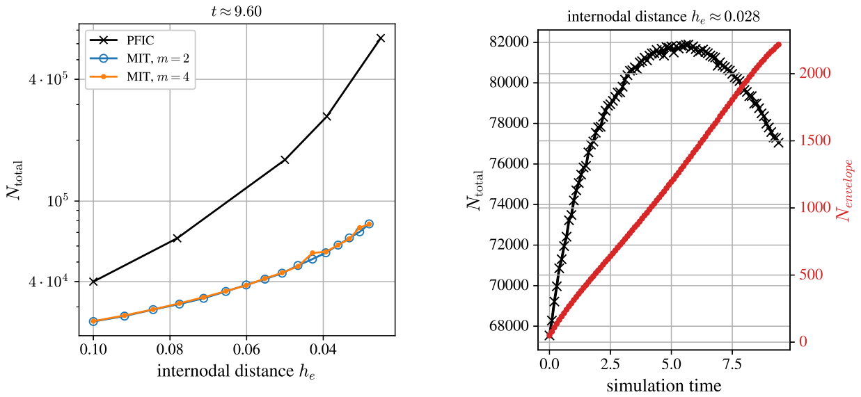
(a) Number of nodes at simulation time t \approx 9.60 with respect to the internodal distance h_e , comparison of MIT and PFIC.
