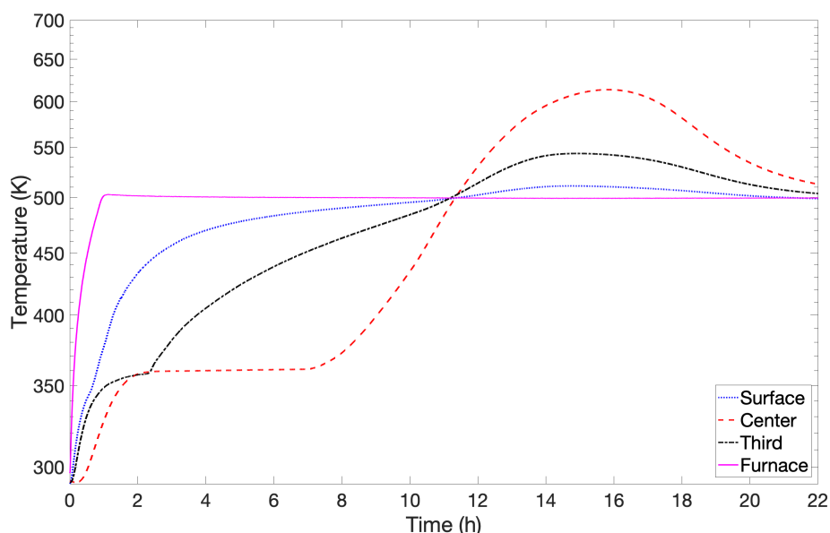
Figure 2: Example of a self-heating test on a soil polluted by hydrocarbons in a 8000 cm 3 basket at 230 °C
