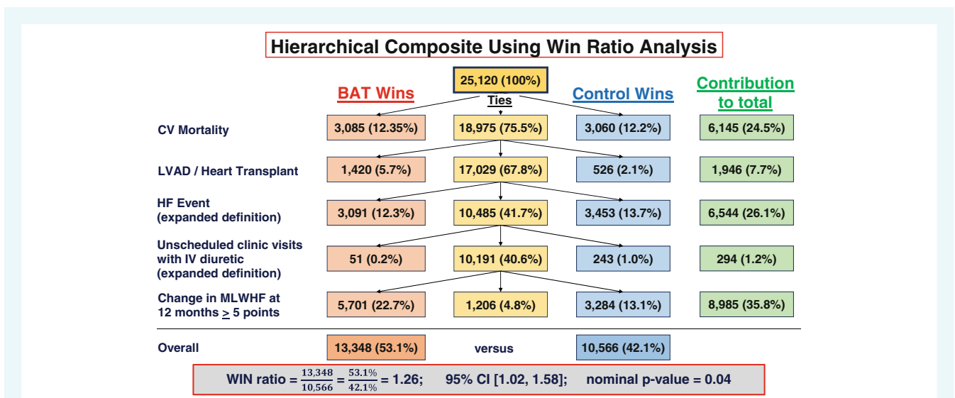
Figure 4 Hierarchical composite using win-ratio analysis. The hierarchical structure applied to the BeAT-HF data used a five level composite (see text for details) and the Finkelstein–Schoenfeld statistical method. The win ratio of 1.26 favoured the baroreceptor activation therapy (BAT) group with 26% more wins in BAT versus control. CI, confidence interval; CV, cardiovascular; HF, heart failure; IV, intravenous; LVAD, left ventricular assist device; MLWHF, Minnesota Living With Heart Failure.
