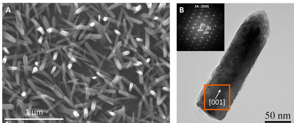
Fig. 1. SEM (A) and TEM (B) micrographs (FFT in inset) of Te nanorods electrodeposited in EOPiPFSI:EOPiPBr 95:5 (mol%). [TeCl 4 ] = 5 mmol·L -1 . T = 100 °C, Q = 0.1C·cm -2 .
