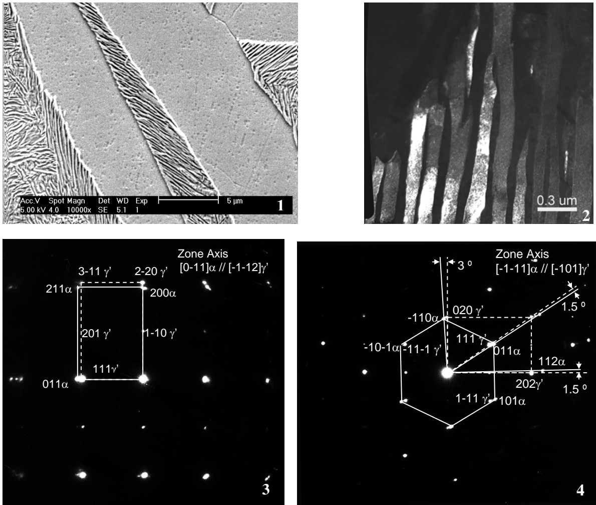
Fig. 1 SEM image of nitrogen pearlite.
