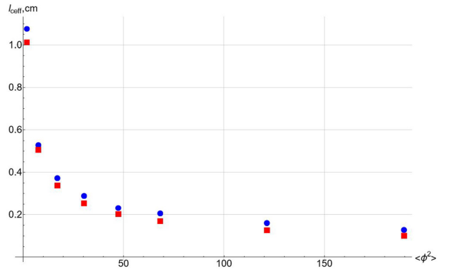
FIG. 2. The signal correlation length l_{eff} vs the signal average phase variation squared, the different points correspond to the different turbulence amplitudes, and the turbulence amplitudes set is shown in Fig. 1. The blue circles represent the numerically evaluated l_{eff} , and the red squares stand for the analytical values. The turbulence spectrum is Gaussian with l_c = 1 cm and the probing beam width \rho = 2 cm.
