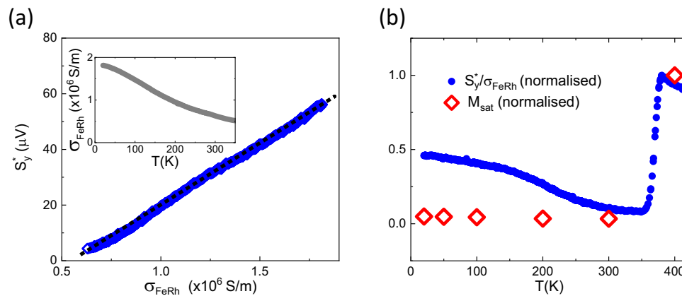
Fig. 3 | Dependence of the THz emission on FeRh conductivity. a S_y^s measured in FeRh-Pt, pumping on the Pt side, as a function of FeRh conductivity, \sigma_{\text{FeRh}} and for a value of the external field of 860 mT. The insert shows the temperature
