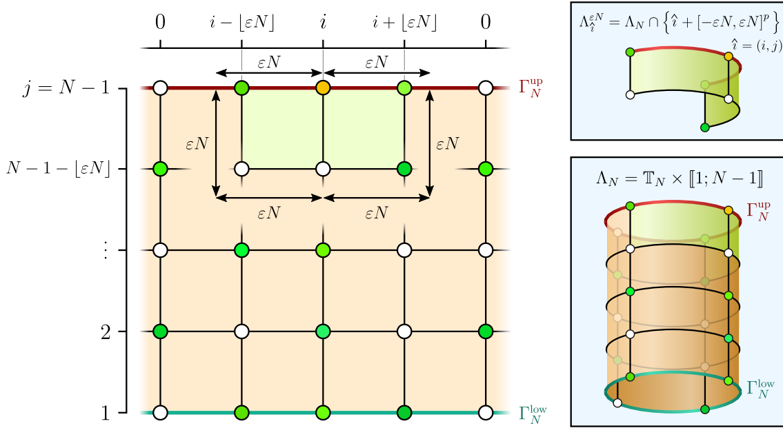
Figure II — The upper Replacement lemma. For \hat{i} = (i, j) \in \Gamma_N^{\text{up}} , we define \Lambda_i^{\varepsilon N} as the intersection between \Lambda_N and the p -dimensional box of range 2\varepsilon N centred on \hat{i} . Notice that for fixed \varepsilon > 0 , the size of the box remains constant at the macroscopic scale. Lemma 4.4 establishes that, as N \rightarrow \infty followed by \varepsilon \rightarrow 0 , the value of \eta(\hat{i}) can be replaced by \eta^{\varepsilon N}(\hat{i}) which is the mean value of \eta inside \Lambda_i^{\varepsilon N} .
