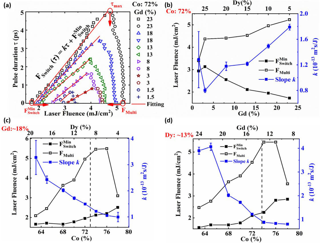
FIG. 4. Evolution of AO-HIS state diagrams for a 10-nm \text{Gd}_x\text{Dy}_{1-x}\text{Co}_y alloy sample. (a) Evolution of the magnetic-state diagrams for various Gd concentrations while the Co concentration is kept constant at x = 72\% , \text{Gd}_y\text{Dy}_{0.28-y}\text{Co}_{0.72} . The parameters F_{\text{Switch}} , F_{\text{Multi}} , and k are extracted from (a) and Figs. S4(a) and S4(b), as a function of Gd and Co concentrations, (b) for a constant Co concentration equal to 72%, (c) for a constant Gd concentration equal to 18%, and (d) for a constant Dy concentration equal to 13%. The dashed lines in (c) and (d) correspond to the compensation point.
