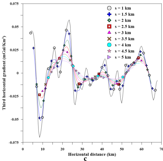
Fig. 7 a Case 1: Geological map for the area including the Seattle Fault System, USA (after Brink et al. 2002). b Observed and predicted gravity anomalies deduced from using the third horizontal gradient method. c Third horizontal derivative anomalies using different s values of b . d Convergence rate of the PSO scheme after applying
