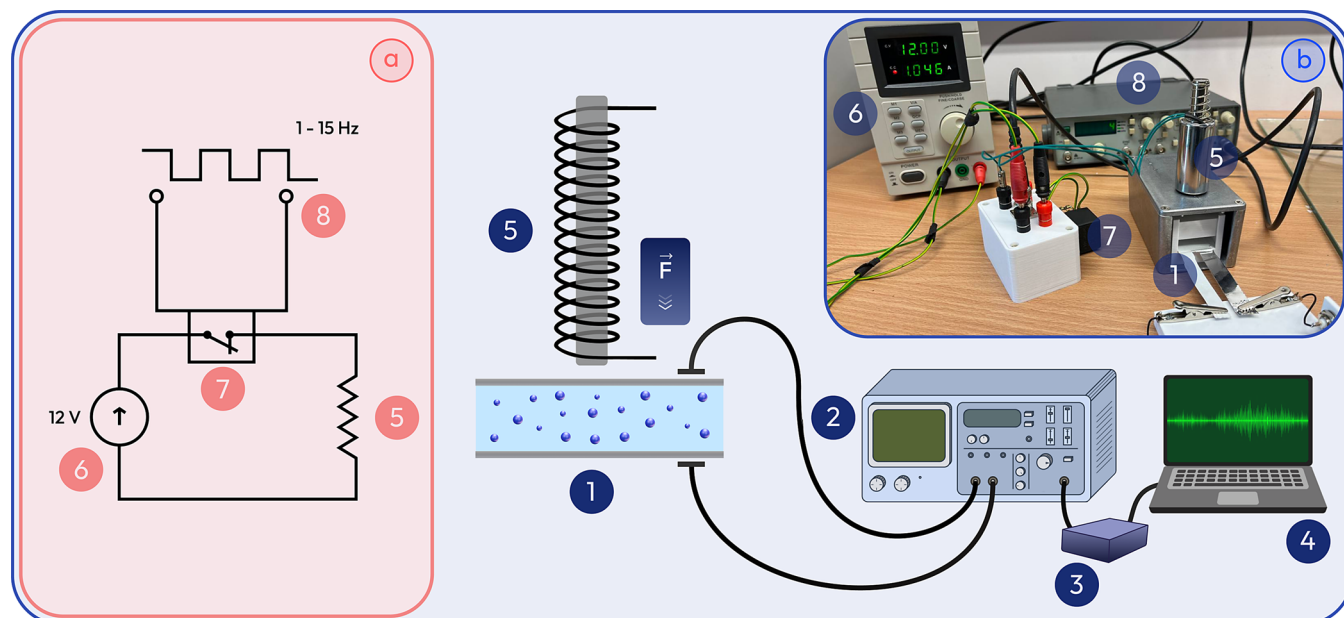
Figure 2. Experimental setup for measuring nanogenerator output characteristics, including (a) electrical diagram of electromagnet powering and (b) photo of its practical implementation: 1 - nanogenerator device (sandwich system of a thin BTO/PDMS composite layer between Al contacts); 2 - oscilloscope; 3 - adapter; 4 - PC; 5 - pushing electromagnet; 6 - DC power supply; 7 - relay; 8 - laboratory generator.
