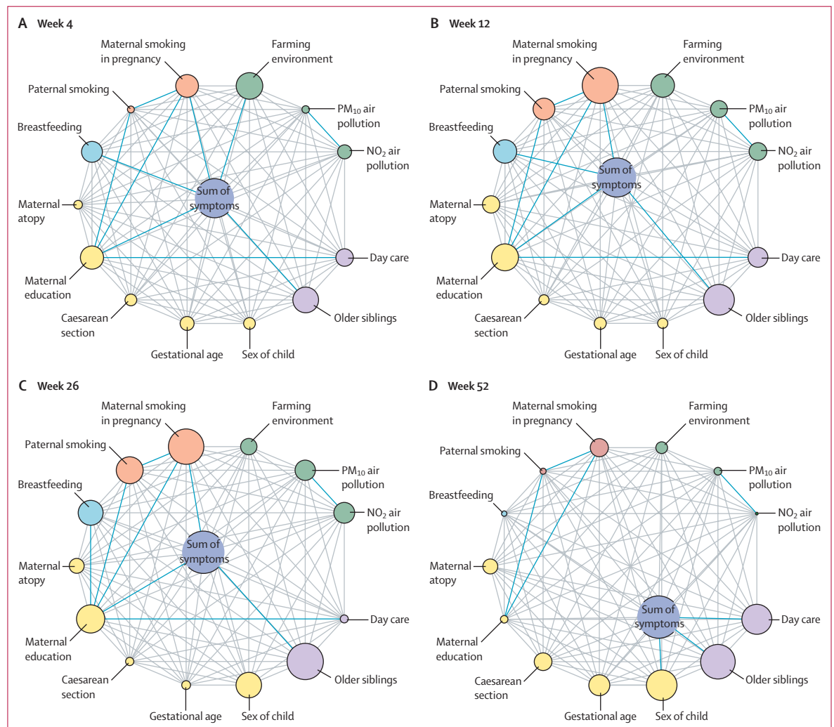
Figure 4: Dynamic host–environment correlation network over the first year of life; the BILD cohort
