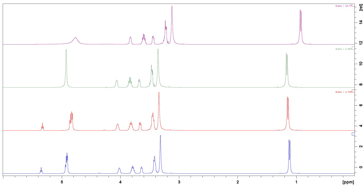
Figure 8. ^1\text{H} NMR spectra of Pr 1:3 (blue), and Pr1:3 + \text{PdCl}_2 (red), Pr 1:3 + \text{AuCl}_3 (green) and Pr 1:3 + \text{AgCl} (purple).
