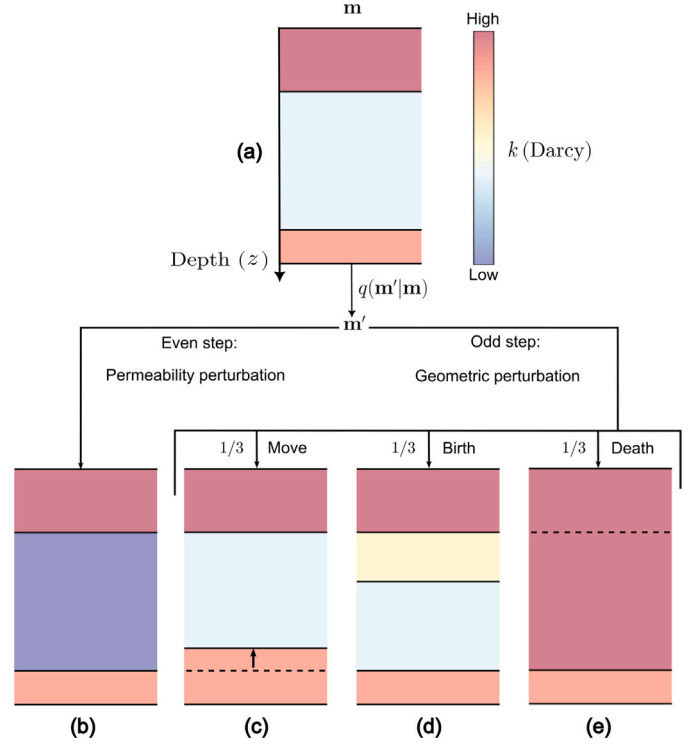
Fig. 3. (a) Current model at the i th iteration of RJMCMC. Four different model perturbations are allowed to generate a candidate model. (b) Change of permeability in a randomly selected layer. (c) Move of a randomly selected layer interface. (d) Birth of a new interface and sampling of the permeability value in the new layer. (e) Death of a randomly selected interface and merge of permeability between neighboring layers.
