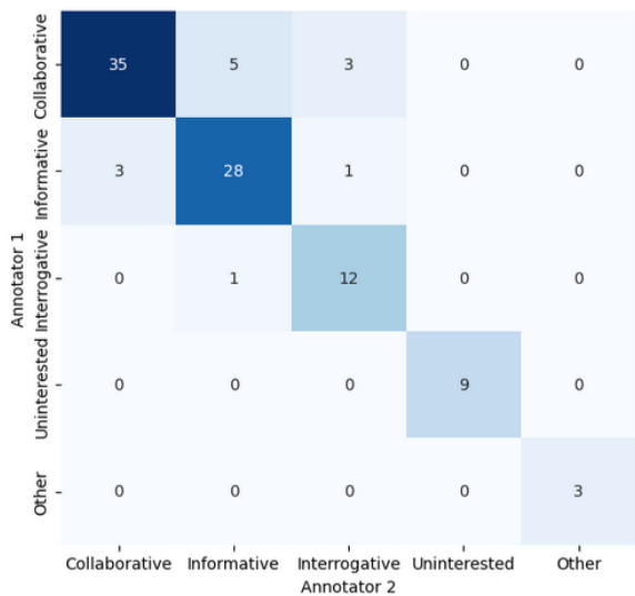
Figure 6: IAA heatmap for discourse acts - 0.857
