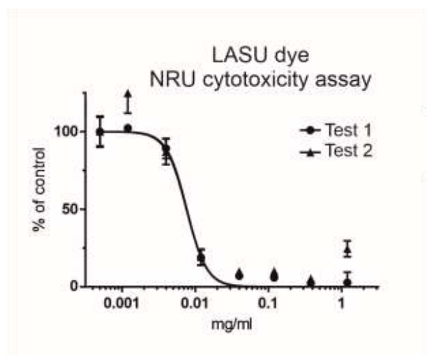
Figure 14. The dose-response effect of LASU phthalocyanine on BALB/c 3T3 fibroblast viability. The assay was performed twice (Test 1 and Test 2) with six replicates of each concentration in both assays.
