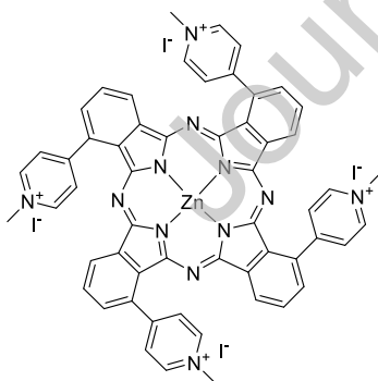
Figure 1. LASU phthalocyanine
