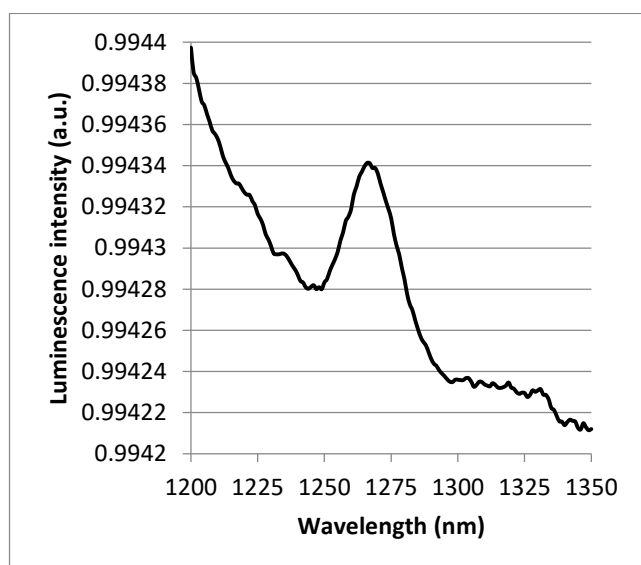
Figure 5. Singlet oxygen luminescence spectra after illumination of cotton upon excitation at 350 nm.
