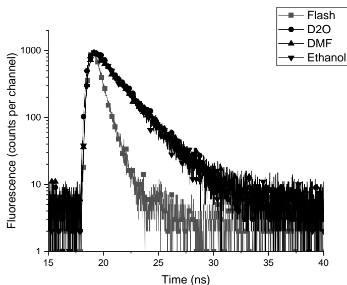
Figure 8: Fluorescence decays of LASU in water, D 2 O, DMF, EtOH and toluene
