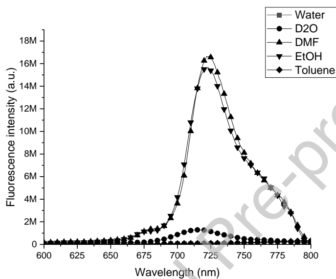
Figure 7. Fluorescence emission spectra of LASU in water, D 2 O, DMF, EtOH and toluene
