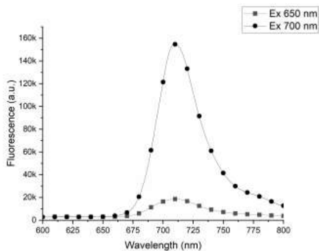
Figure 11: Fluorescence emission spectra of LASU in the textile upon excitation at 650 nm (squares) and 700 nm (circles)
