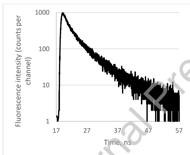
Figure 4. Fluorescence decay of cotton upon excitation at 408 nm
