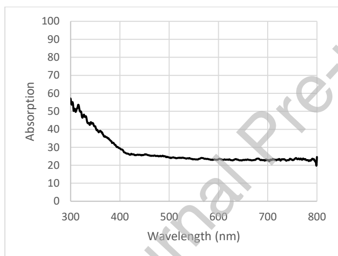
Figure 2. Cotton absorption spectrum
