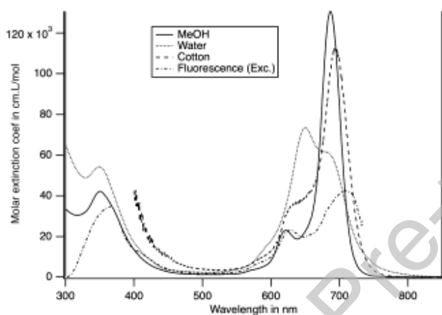
Figure 10. Absorption and fluorescence of LASU on cotton.
