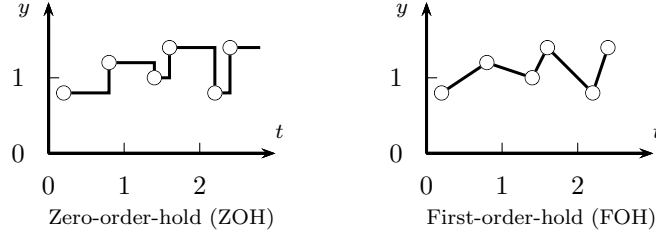
Figure 4.2: Reconstruction of CT signals from the sampled data for two intersample behavior assumptions.
