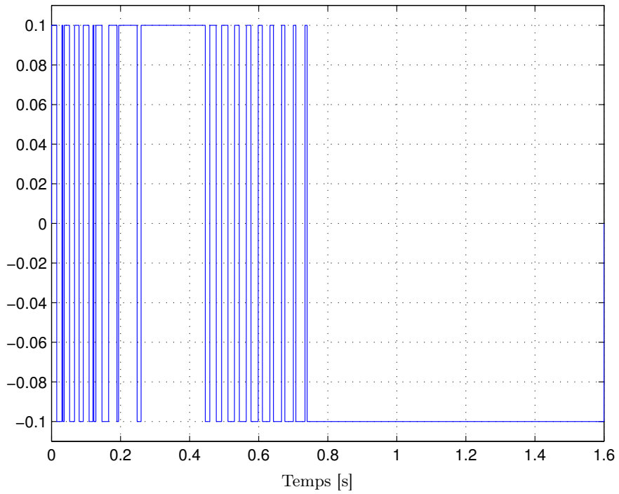
FIGURE 4.10 – Commande u_1(t) .
