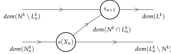
Figure 5.1: Inductive construction
