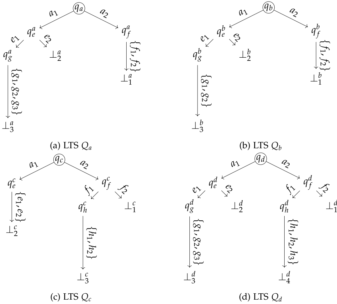
Figure 3.17: Sub LTS(s)
