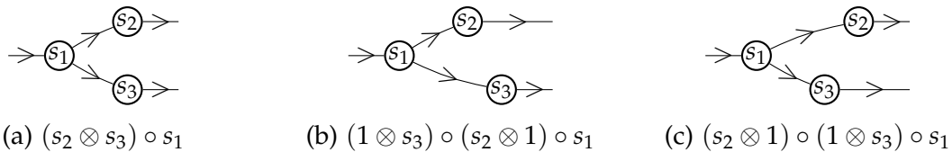
Figure 5.3: String diagrams
