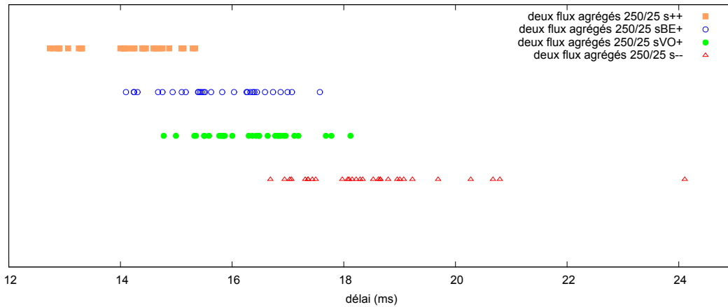
Figure 3.70 – Délai maximum, flux best-effort , e250v_{e25} (sans pertes)
