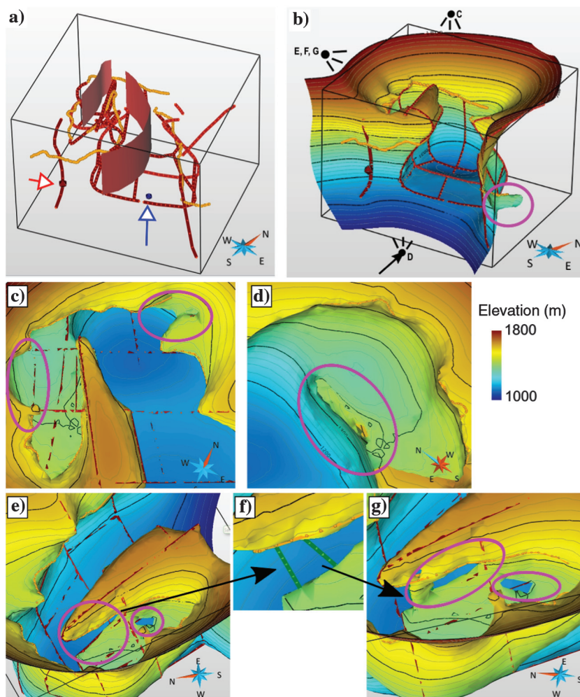
Figure 8. Implicit modeling of the salt surface with inequality constraints. (a) Additional information used to impose the surface polarity: two surfaces are defined inside the minibasin as well as one point (in red). They are attached to a greater than constraint (Frank et al., 2007). One point is used at depth (in blue) to define the other side of the surface using a less than constraint. (b) Result obtained using a volumetric tessellation of 30 m resolution. (c) Top view and magnification of the model (b). (d) Bottom view on the central diapir showing the local fusion of the two sides and the artifacts due to mesh resolution. (e) Side view of the central diapir highlighting the unwanted “hole” in the salt. (f) Additional curves used to force the interpolation to close this hole and corresponding result (g).
