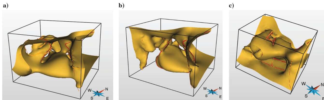
Figure 7. Implicit modeling of the salt surface with digitized curve constraints alone. Panels (a–c) show models built with volumetric mesh resolutions of (a) 10, (b) 20, and (c) 30 m.
