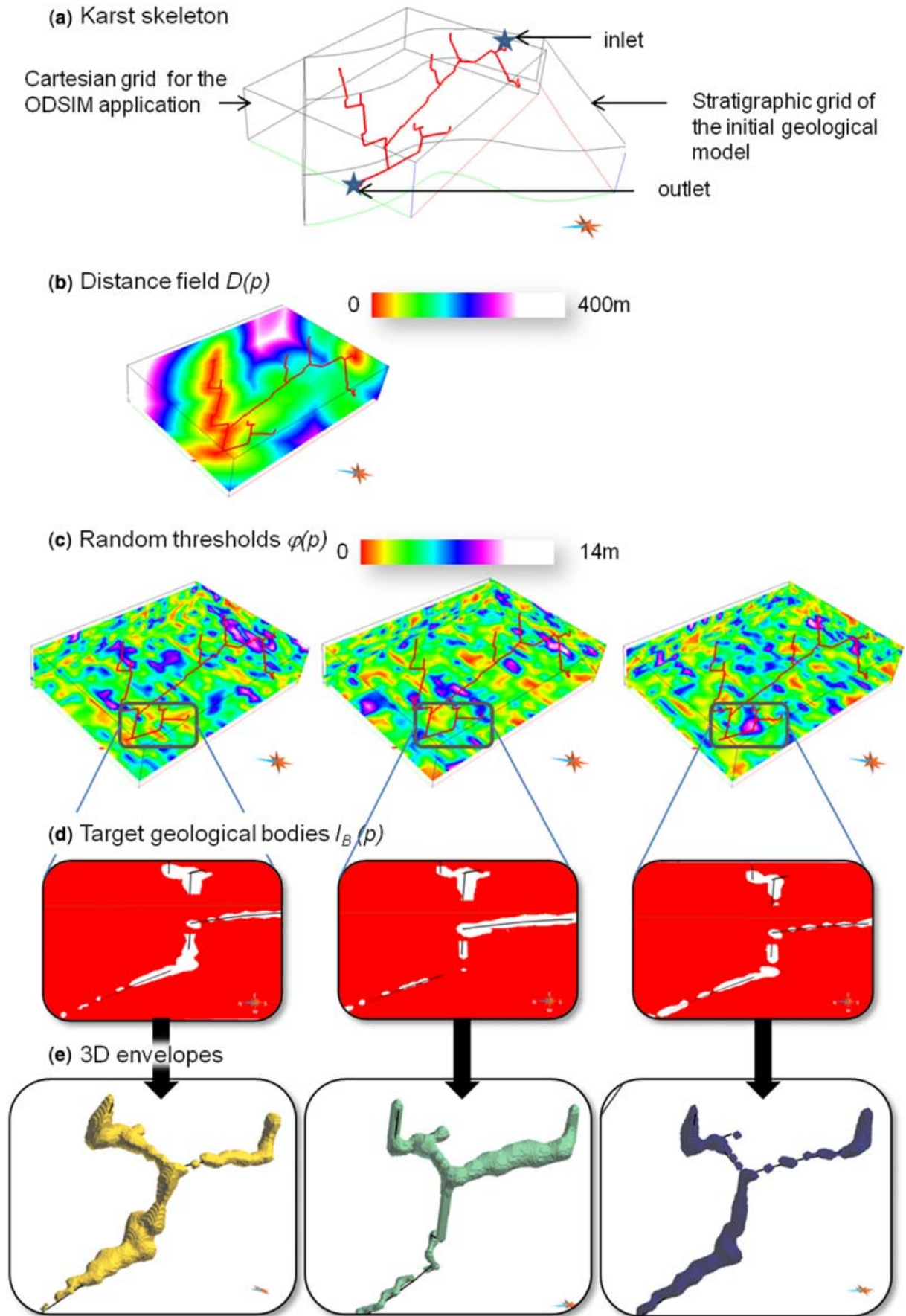
Fig. 10. Application of the ODSIM method to the reference skeleton.
