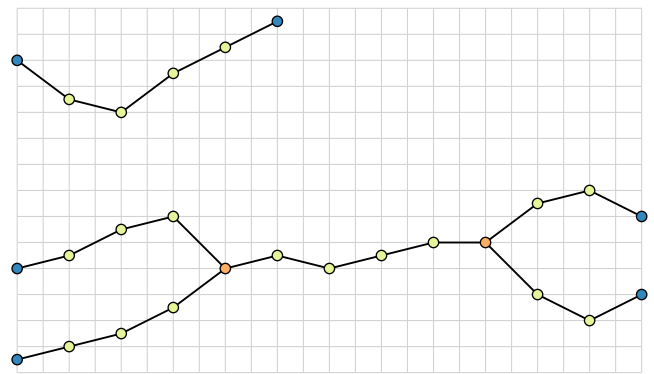
Node of degree 1 (blue), Node of degree 2 (yellow), Node of degree 3 (orange), Node of degree 1 along a border (blue).
