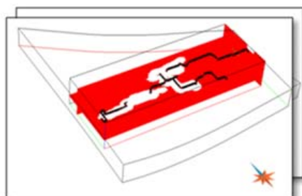
Fig. 2. General workflow for stochastic 3D karst simulation.
