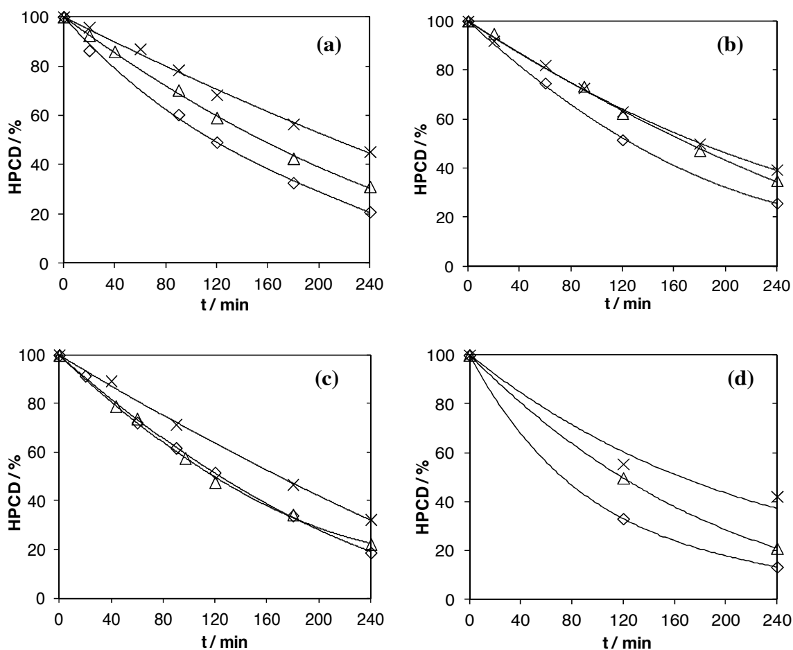
Fig. 5.2. Effect of applied current intensity (500 mA ( \times ), 1000 mA ( \Delta ) and 2000 mA ( \diamond )) with different anode materials and different kind of treatment (EF-Pt (a), EF-DSA (b), EF-BDD (c) and AO-BDD (d)) on HPCD ( 9 \text{ g L}^{-1} ) degradation in the presence of PHE ( 0.09 \text{ mM} ).
