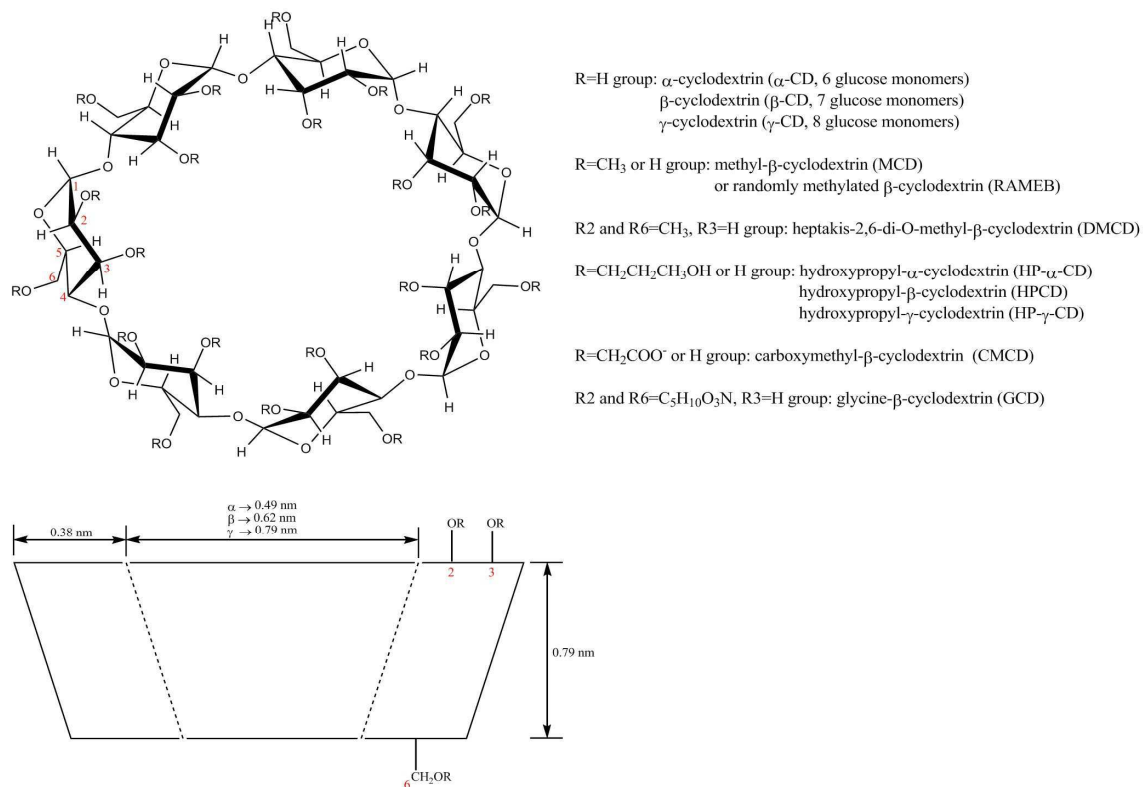
Fig. 2.1. Structure of some native and derivative cyclodextrins used in SW/SF processes.
