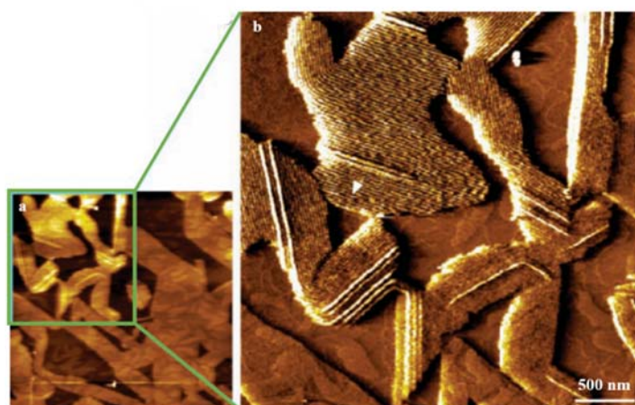
Figure 1-8. Ripples in a l_o/l_d phase coexistence of a (1:1) DMPC/DSPC double bilayer. a) Height mode AFM image at 32.5 °C. b) Deflection mode zoom of a , showing ripples in the l_o phase domain (white arrow) [48].
