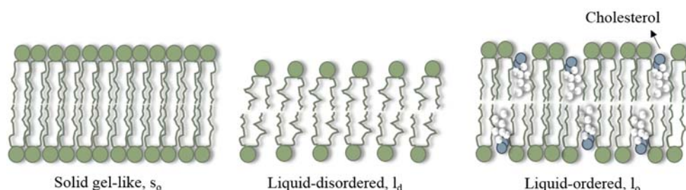
Figure 1-7. Different membrane phases of phospholipid bilayers; solid gel-like ( s_o ), liquid-disordered ( l_d ) and liquid-ordered ( l_o ) containing cholesterol (drawn based on [11]).
