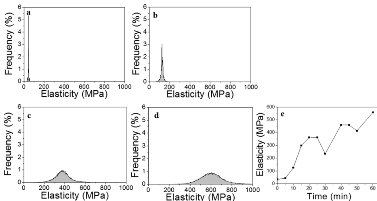
Figure 3-28. Distributions of Lipid A/LPS St SLB elasticity in TRIS buffer a) before, b) 0 min, c) 20 min and d) 60 min after bCAT (60 \mu M) injection. e) Elasticity within time.
