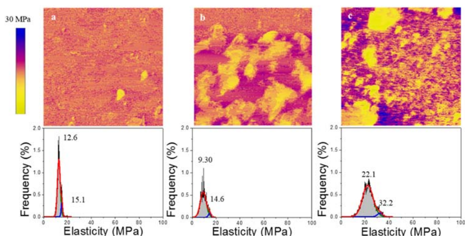
Figure 3-22. Derjaguin-Muller-Toporov (DMT) modulus images (top panel) and elasticity distributions (bottom panel) of supported DPPC/DOPC SLBs in TRIS buffer a) before, b) 5 min and c) 60 min after bCAT (60 \mu M) injection.
