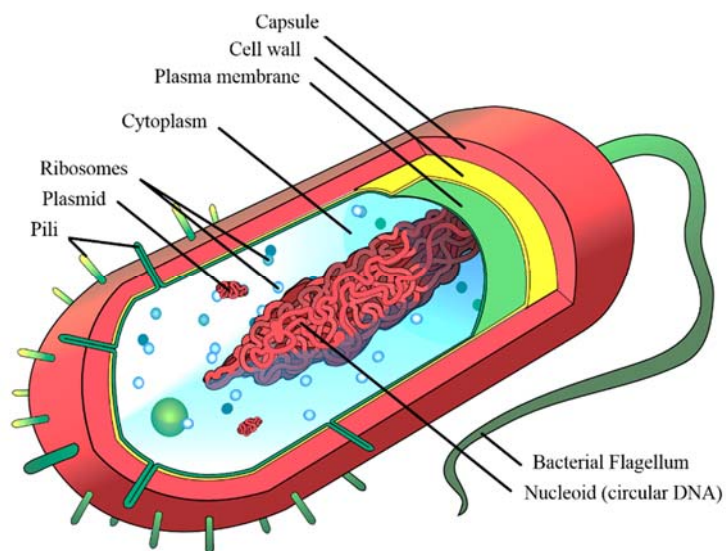
Figure 1-11. General structure of a bacteria with its genetic material floating in the cytoplasm bounded by the bacterial cell wall to which several external structures such as pili and flagella are attached.
