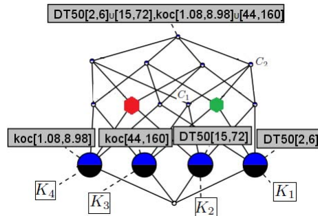
Figure 5: Concept lattice built from Table 4
