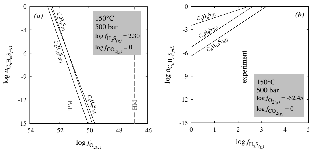
Figure 2.20. \log f_{\text{O}_2(g)} - \log a_{\text{C}_n\text{H}_m\text{S}_p(l)} and \log f_{\text{H}_2\text{S}(g)} - \log a_{\text{C}_n\text{H}_m\text{S}_p(l)} diagrams showing the relative abundances of thiacyclopentane ( \text{C}_4\text{H}_8\text{S}(l) ), 1,2-dithiacyclohexane ( \text{C}_4\text{H}_8\text{S}_2(l) ), and 1,4-butanedithiol ( \text{C}_4\text{H}_{10}\text{S}_2(l) ) for Experiments 2a and 2b.
