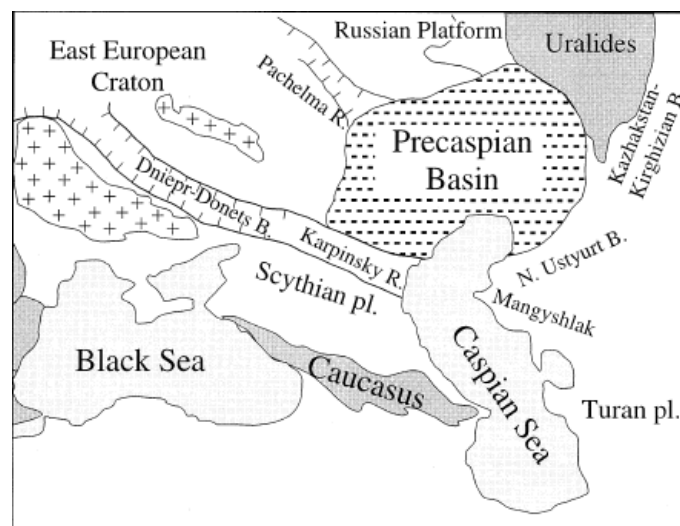
Figure 3.2. Location of the Pre-Caspian Basin and main regional tectonic units (Brunet et al., 1999).
