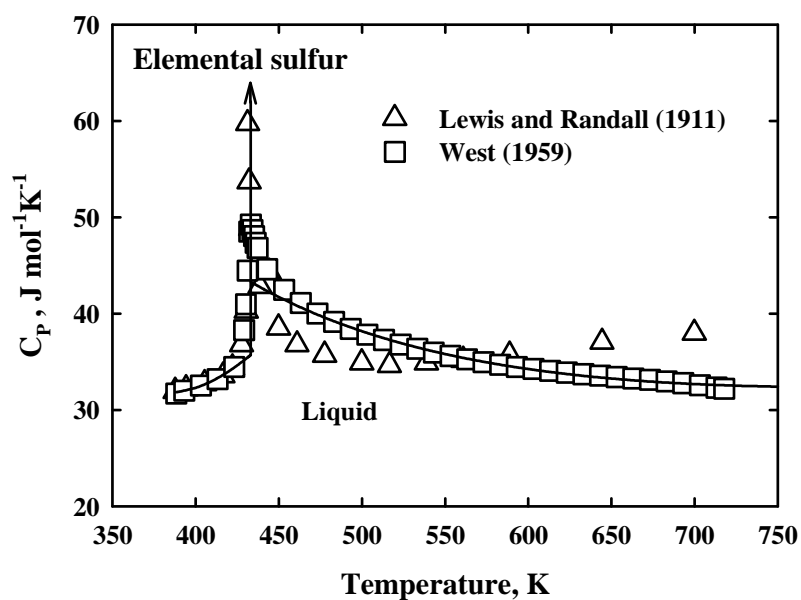
Figure 1.6. Standard molal heat capacity of liquid sulfur as a function of temperature at ~ 1 bar. The curves represent regressions with Equation (1.10) of the data represented by the symbols and are consistent with the a , b , and c coefficients listed in Table A1 for liquid sulfur – see text.
