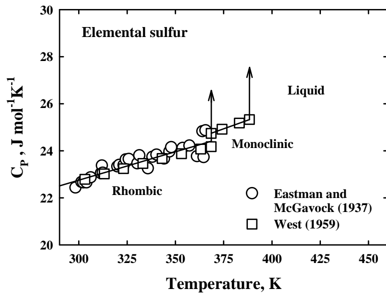
Figure 1.5. Standard molal heat capacity of crystalline sulfur as a function of temperature at ~ 1 bar. The straight lines represent regressions with Equation (1.10) of the data represented by the symbols and are consistent with the a , b , and c coefficients listed in Table A1 for rhombic and monoclinic sulfur.
