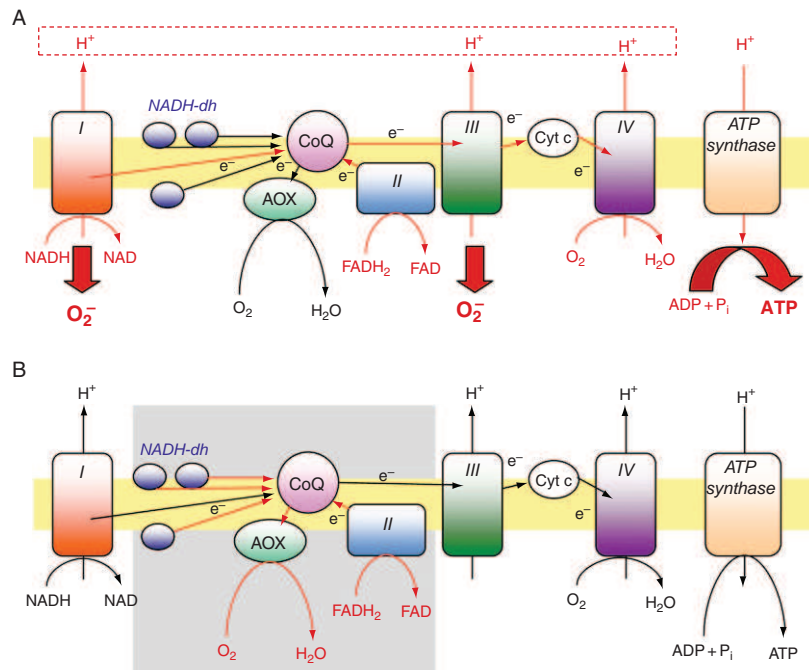
Fig. 3. Regulation of the mitochondrial electron transport chain of P. chrysosporium grown in a ligninolytic condition compared to a control condition. (A) When the intracellular oxidative stress is low, all the classical mitochondrial complexes are involved in creating the proton gradient required to produce ATP. Complexes I and III are responsible for most of the superoxide production. To maintain a nontoxic amount of superoxide inside the cell, some detoxifying enzymes function in their degradation. (B) When there is a high oxidative stress, another level of regulation involves alternative mitochondrial pathways to bypass complexes I and III and limit ROS production. Red arrows indicate the preferential pathway in conditions (A) and (B).
