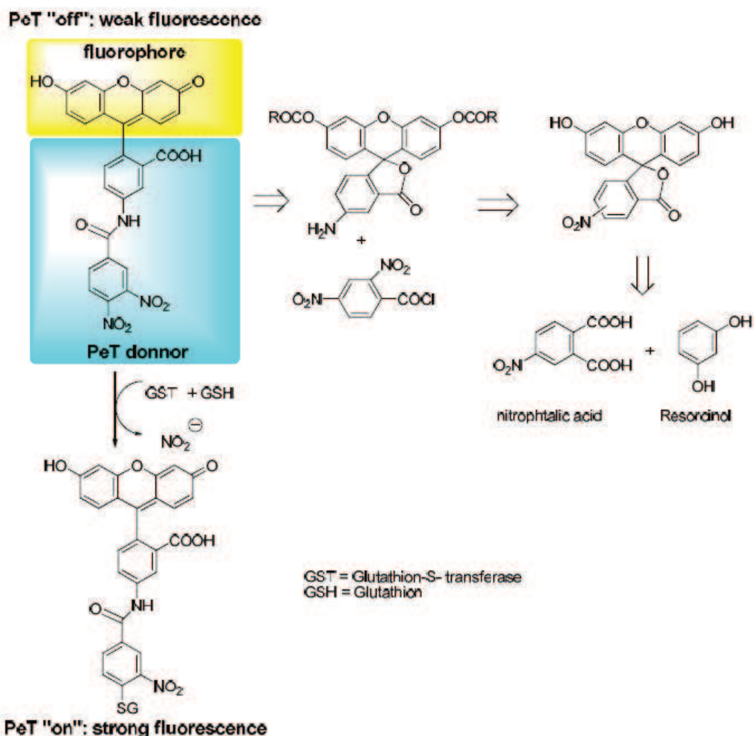
Figure 17: Synthesis and mode of action of GST fluorogenic probes (Fujikawa et al., 2008)
