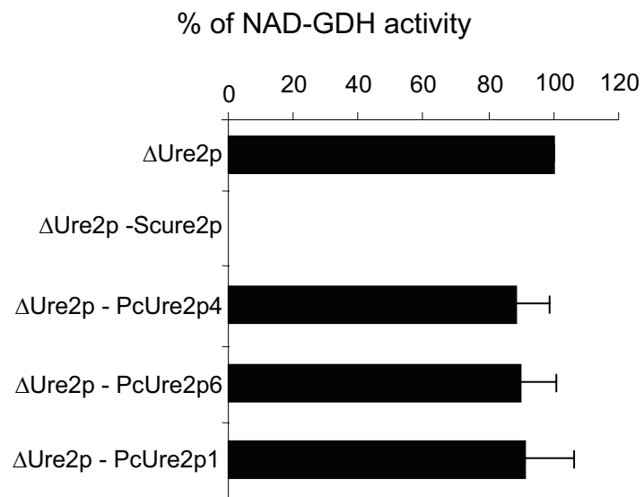
Fig. 5: NAD-GDH activity in the transformed yeast strains. \Delta\text{Ure2p} is the mutant strain transformed with the empty pYes2 vector. The other strains correspond to the mutant transformed with the pYes2 vector harbouring either the endogenic ScUre2p or the heterologous PcUre2p4, 6 and 1. The results are expressed as percentages of the higher activity found for the mutant \Delta\text{Ure2p} .
