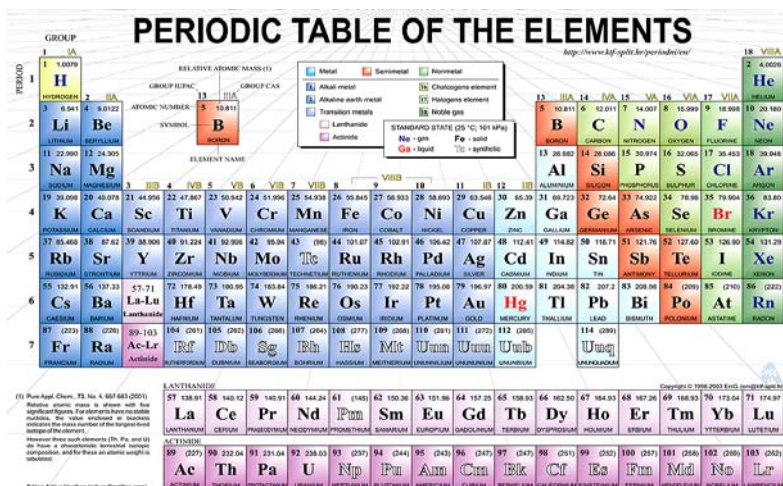
Figure 1. Periodic table of the elements. Metal elements are in blue, semi-metal (metalloid) elements are in orange and non-metal elements are in green ( http://blogs.4j.lane.edu/taylork/2010/06/01/metals-this-week-in-science-june-1-june-4/ ).
