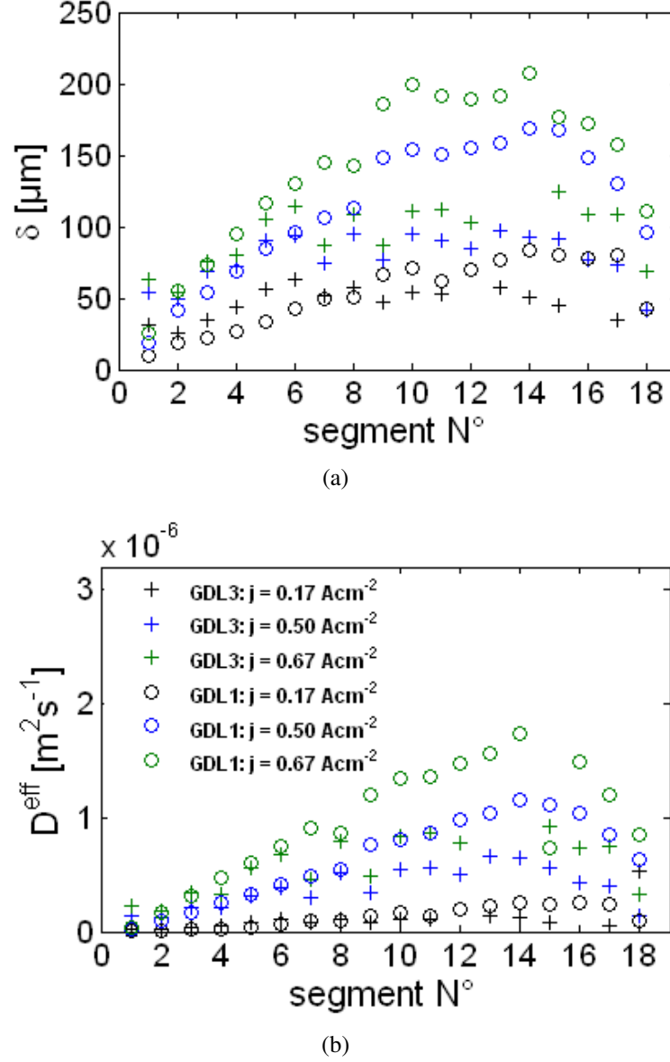
Figure 6.15: Diffusion parameters identified with GDL 1 ( \delta_{\text{GDL1}} = 235 \mu\text{m} with MPL) and GDL 3 ( \delta_{\text{GDL3}} = 190 \mu\text{m} without MPL) at different current densities: (a) diffusion thickness \delta , (b) effective diffusion coefficient D^{\text{eff}} .
