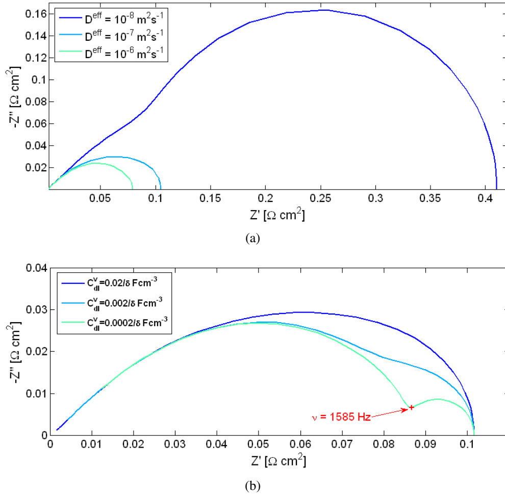
Figure 4.11: Impedance spectra determined numerically with the finite-difference method in the operating conditions of Table 4.3: (a) for different values of the effective diffusivity; C_{\text{dl}}^{\text{v}} = 0.02/\delta \text{ F cm}^{-3} and (b) for different values of the double-layer capacity; D^{\text{eff}} = 10^{-7} \text{ m}^2 \text{ s}^{-1} . Even for important diffusion losses ( D^{\text{eff}} = 10^{-8} \text{ m}^2 \text{ s}^{-1} ), there is no clear separation between the capacitive and diffusive loops, except for very low values of the double-layer capacity. However, this separation does only arise in the high frequency regime.
