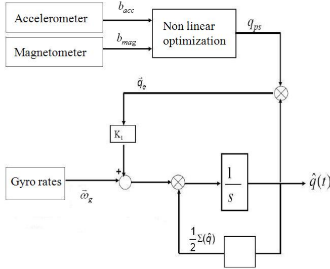
FIGURE 6.10 – Attitude estimation
