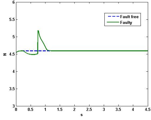
FIGURE 6.16 – Total thrust generated by four motors
