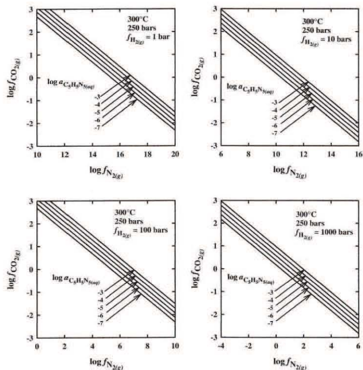
Fig. 5 Logarithmic f_{\text{N}_{2(g)}} - f_{\text{CO}_{2(g)}} fugacity diagrams at 300°C and 250 bars at fixed f_{\text{H}_{2(g)}} values. The straight lines in the diagram correspond to logarithmic contours of the activity of adenine computed from Eq. 9
