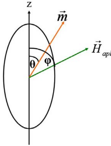
Figure 1.12: Ellipsoid with easy axis along the z-axis. \theta represents the angle between the magnetic moment and the z-axis. \phi represents the angle between the applied field and the z-axis.
