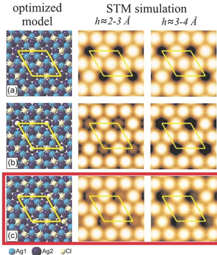
Figure 3.16. Structural models and Tersoff-Hamann simulated STM images for the (3 \times 3) phase calculated for two different tip heights: 2–3 Å and 3–4 Å. (a) The model without atoms in the holes (coverage 0.33 ML); (b) the model with one Cl atom per hole placed in symmetrical position (coverage 0.44 ML); and (c) the equilibrium structure with one Cl atom per hole shifted off-center by 0.7 Å in the direction of the close-packed atomic rows of Ag(111) surface (coverage 0.44 ML)
