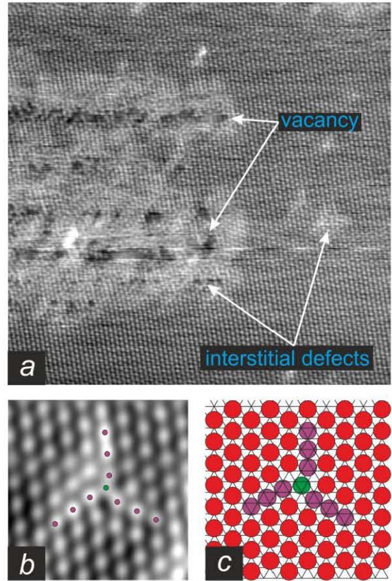
Figure 5.5 (a) Surface region ( 250\times 250 \text{ \AA}^2 , 5K) with chlorine (\sqrt{3}\times\sqrt{3})R30^\circ structure at low temperature after puls-increasement of bias voltage and artificial preparation of interstitial defects (see text for details). (b) STM image ( 40\times 40 \text{ \AA}^2 , 5K) of an interstitial defect. (c) Structural model of an interstitial defect – experiments were done at 5K
