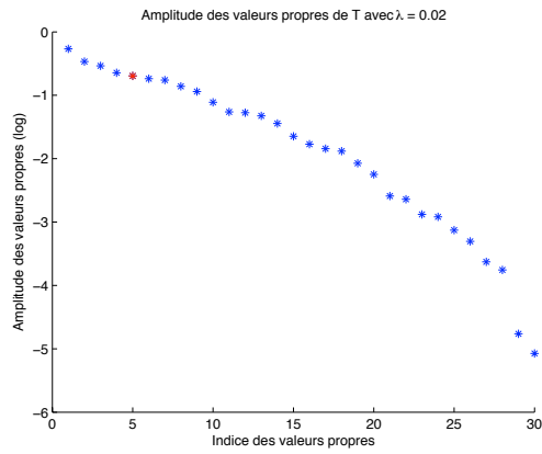
(a) \lambda = 0.02 (= \delta)
