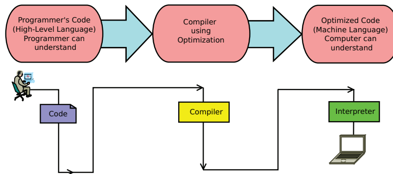
Figure 2.1: Compiler Interaction
