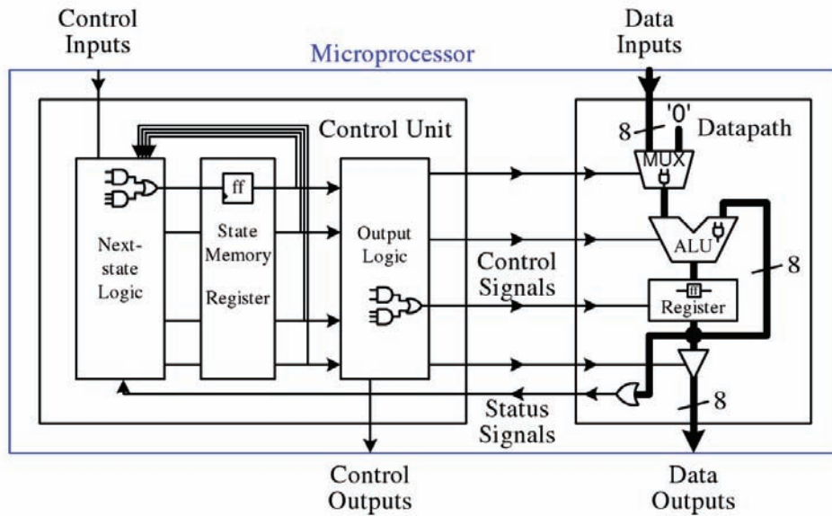
Figure 2.2: Microprocessor
