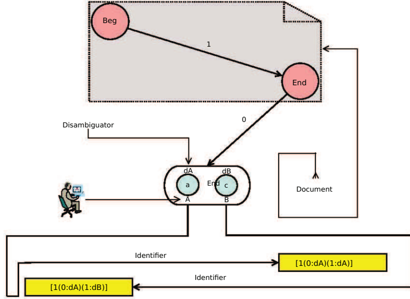
Figure 1.3: Generating POSID
