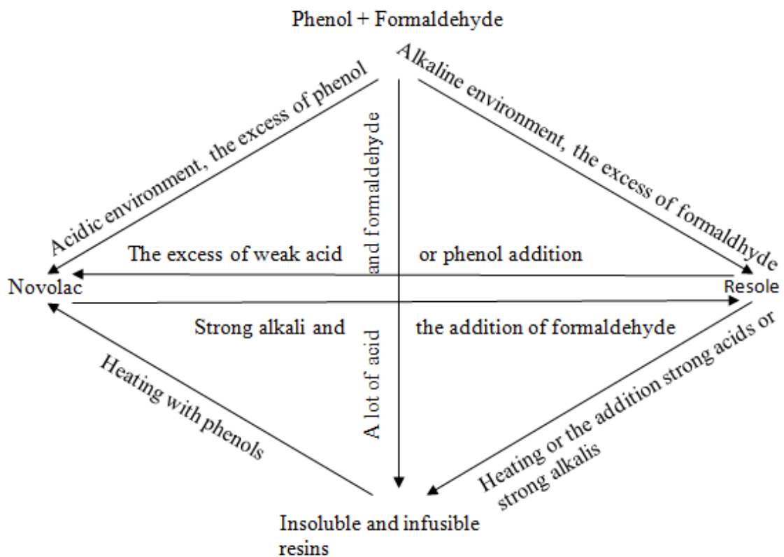
Fig. 11. Pathways of Phenol-Formaldehyde adhesives preparation [26].
