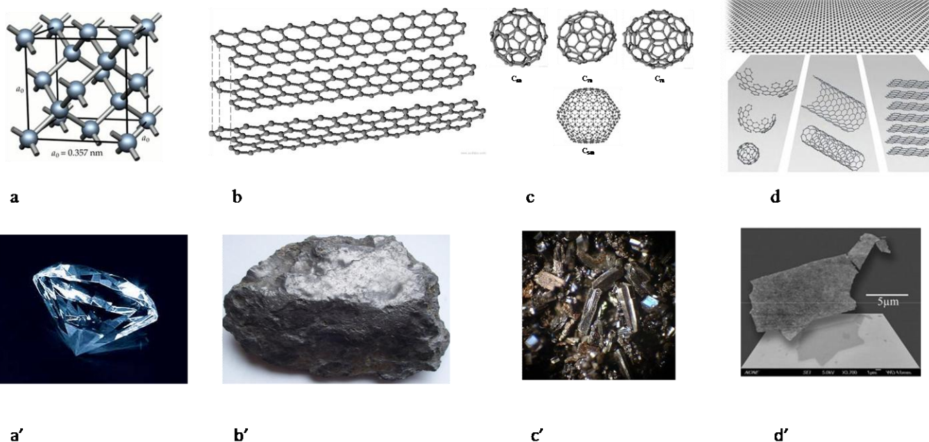
Fig. 24. Allotropes of carbon: a,a') diamond; b,b') graphite; c,c') fullerenes; d,d') graphene.
