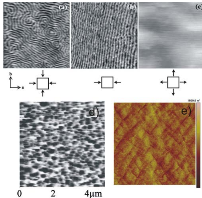
Figure 3.8: MFM images of La_{0.7}Sr_{0.3}MnO_3 thin films, taken in zero applied field at room temperature, on various substrates of (a) LAO, (b) NGO, and (c) STO. The scan size is 4\mu m \times 4\mu m . Taken from [20]. MFM images of LSMO thin films deposited on LAO (d) substrates recorded at RT without an external field. The scan size is 5\mu m \times 5\mu m . Taken from [22]. (e) AFM image with a NiCo MFM tip shows the surface steps on a 20 nm La_{0.67}Sr_{0.33}MnO_3 film on a SrTiO_3 substrate. The scan size is 4\mu m \times 4\mu m in an applied magnetic field of 5.6kA/m. Taken from [31].
