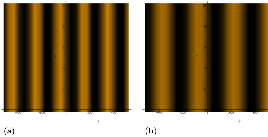
Figure 4.5: Density plot representation of the \partial^2 H_d^{z,total} (a) for p=100 nm, (b) p=150 nm. Following the equation 4.12, the force between a magnetized MFM tip and the magnetic distribution will be proportional to this quantity. This result will roughly qualitatively simulate the MFM contrast of a perpendicular magnetization stripe structure.
