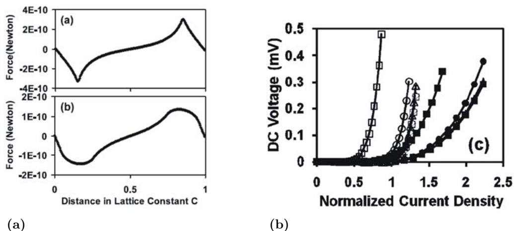
Figure 1.14: (a) Pinning forces calculated for (a) \xi = 2 nm and (b) \xi = 30 nm. (b) IV curves under various fields for the reference sample (open symbols) and for the sample with magnetic dots grown on top (solid symbols). The measurements were performed at T_c - 5.5 K. Taken from [18].
