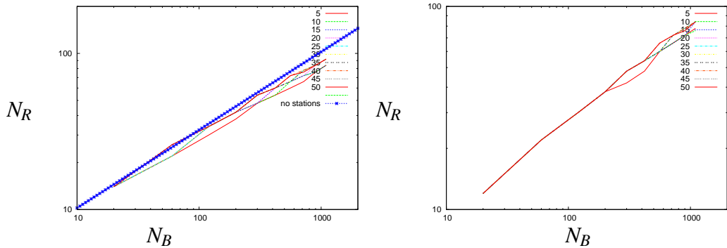
Figure 5.11: The optimal number of routes N_{R_o} as a function of the number of buses N_B , while the number of stations N_S is optimal. Different lines represent different chosen radii r . On the first plot the optimal values are searched as to minimise the average overall time T , while on the second plot we maximise the average overall velocity V .
