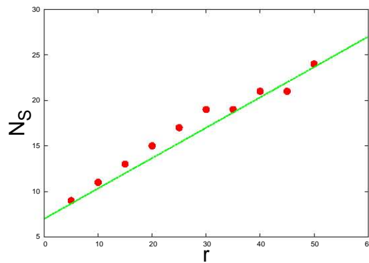
Figure 5.10: The maximal optimal number of stations N_{S_o} as a function of the radius of the city r , while the number of routes N_R is optimal. Optimal values are searched as to minimise the average overall time T
