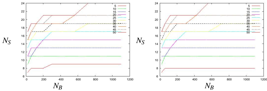
Figure 5.9: The optimal number of stations N_{S_o} as a function of the number of buses N_B , while the number of routes N_R is optimal. Different lines represent different chosen radii r . On the first plot the optimal values are searched as to minimise the average overall time T , while on the second plot we maximise the average overall velocity V .
